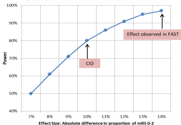
Power by Effect Size as Difference in proportion of mRS 0-2 (treatment-control) at N=388/\text{group} , \alpha=0.05 two-sided, control proportion is 40%
